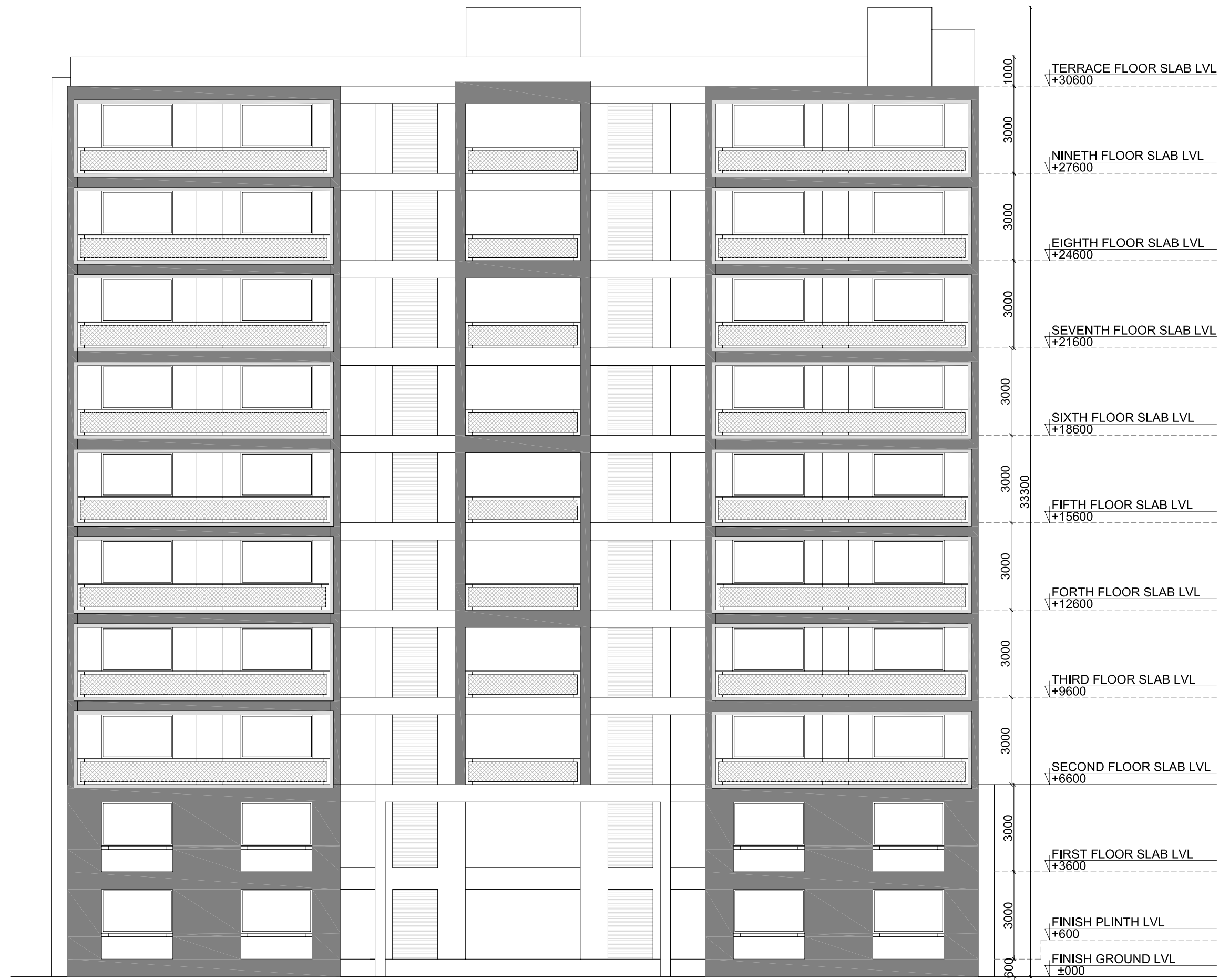
FRONT ELEVATION
